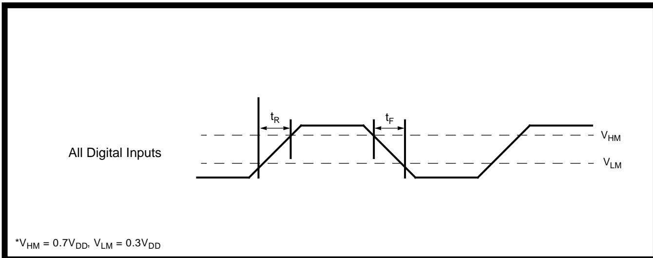
Figure 15 - Digital Signal Input Rise/Fall Times
