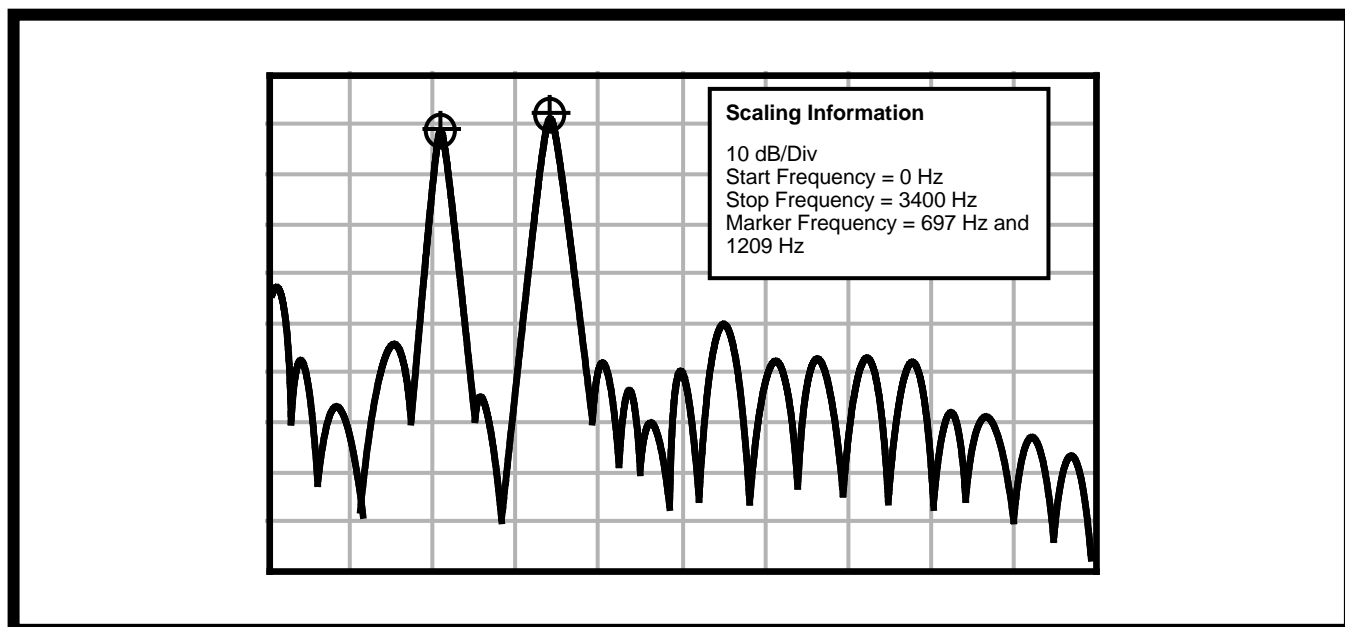
Figure 10 - Spectrum Plot
