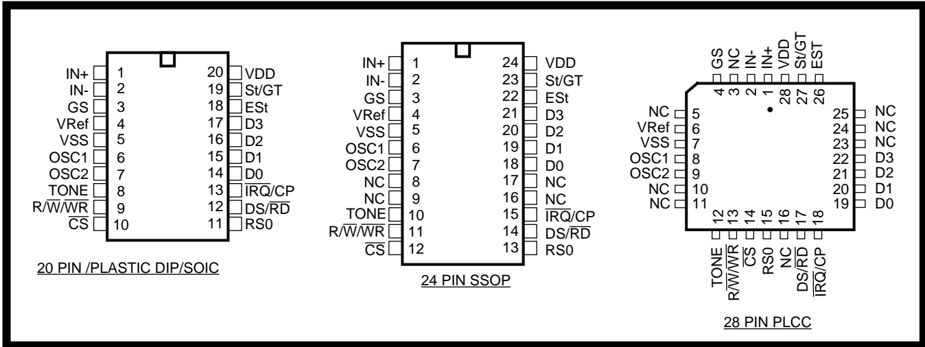
Figure 2 - Pin Connections
